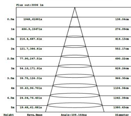
Horizontal illuminance
